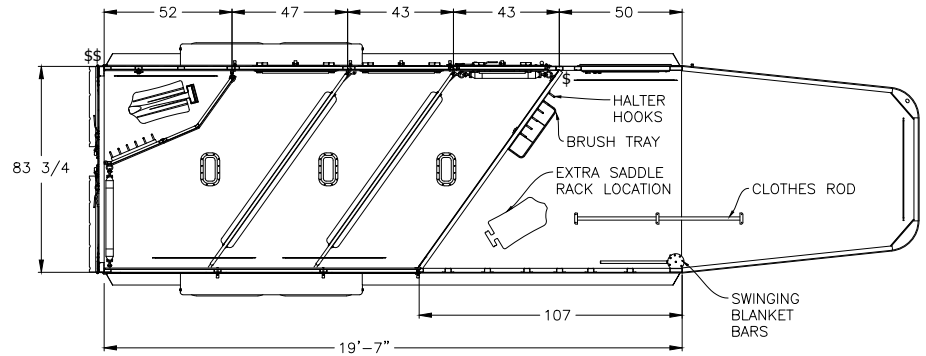
Floorplan shown: 3H with 50" dressing room.
