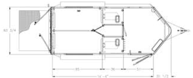
Floorplan: 7442 with 51" dressing room and walk thru door.
