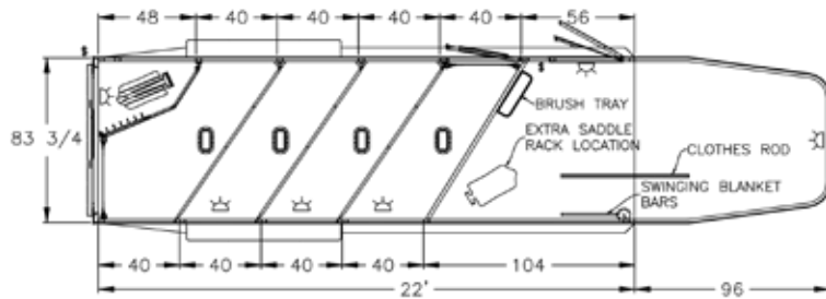
Floorplan: 4-horse model.
