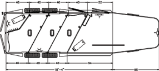
Floorplan: 3-horse with 52" dressing room.
