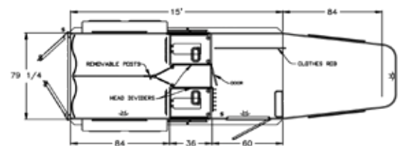
Floorplan: 2-horse with 60" dressing room & mangers.
