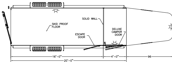
Floorplan: 20' length with straight wall.
