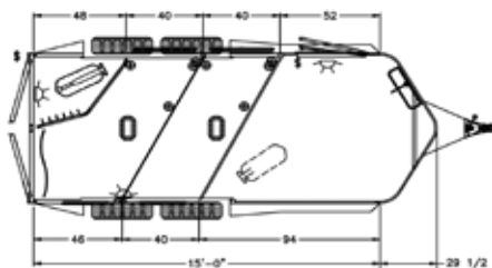
Floorplan: 2-horse with 52" dressing room, 7' width and 40" stalls.
