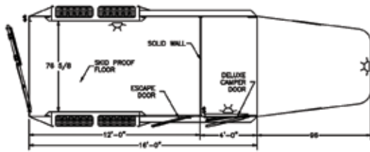
Floorplan: 16' length with straight wall.
