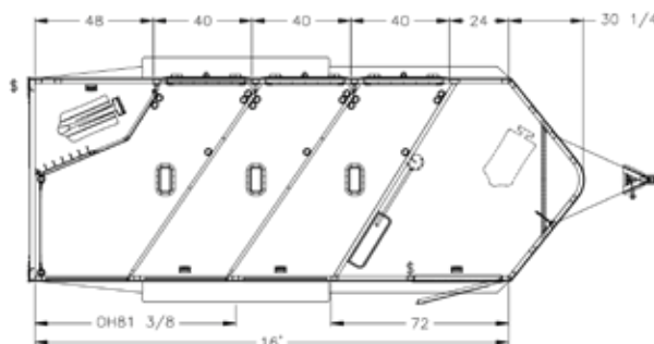
Floorplan: 3H with 24" dressing room.
