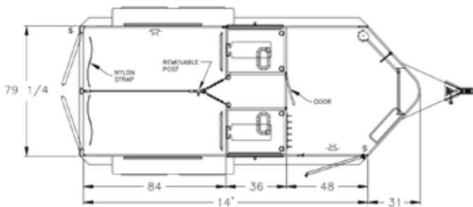
Floorplan: 48" dressing room with mangers & walk-through.
